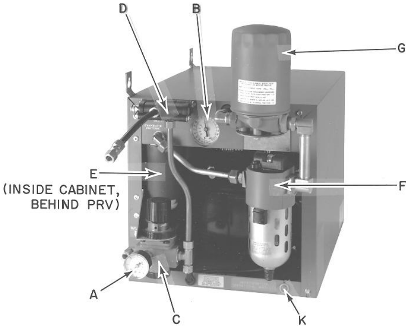
Figure 15: Repair Parts (See Table 3)
