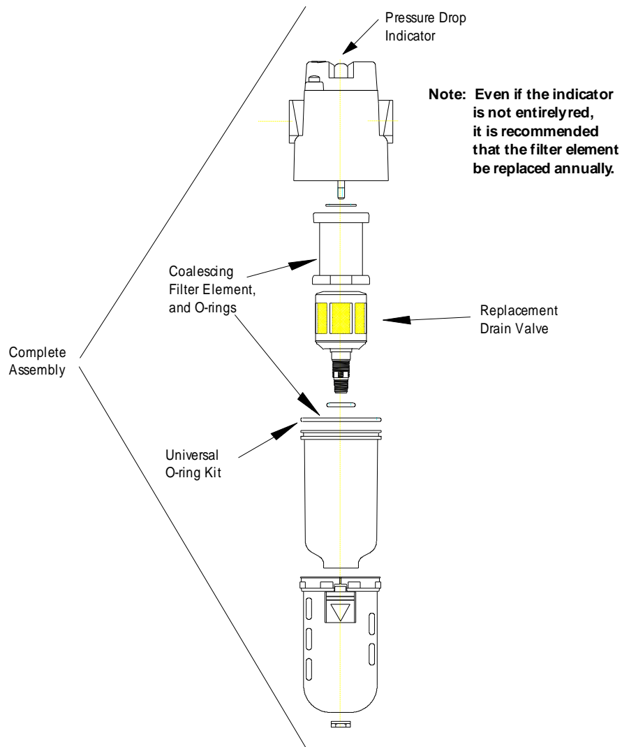
Figure 7: Coalescing Oil Removal Filter
